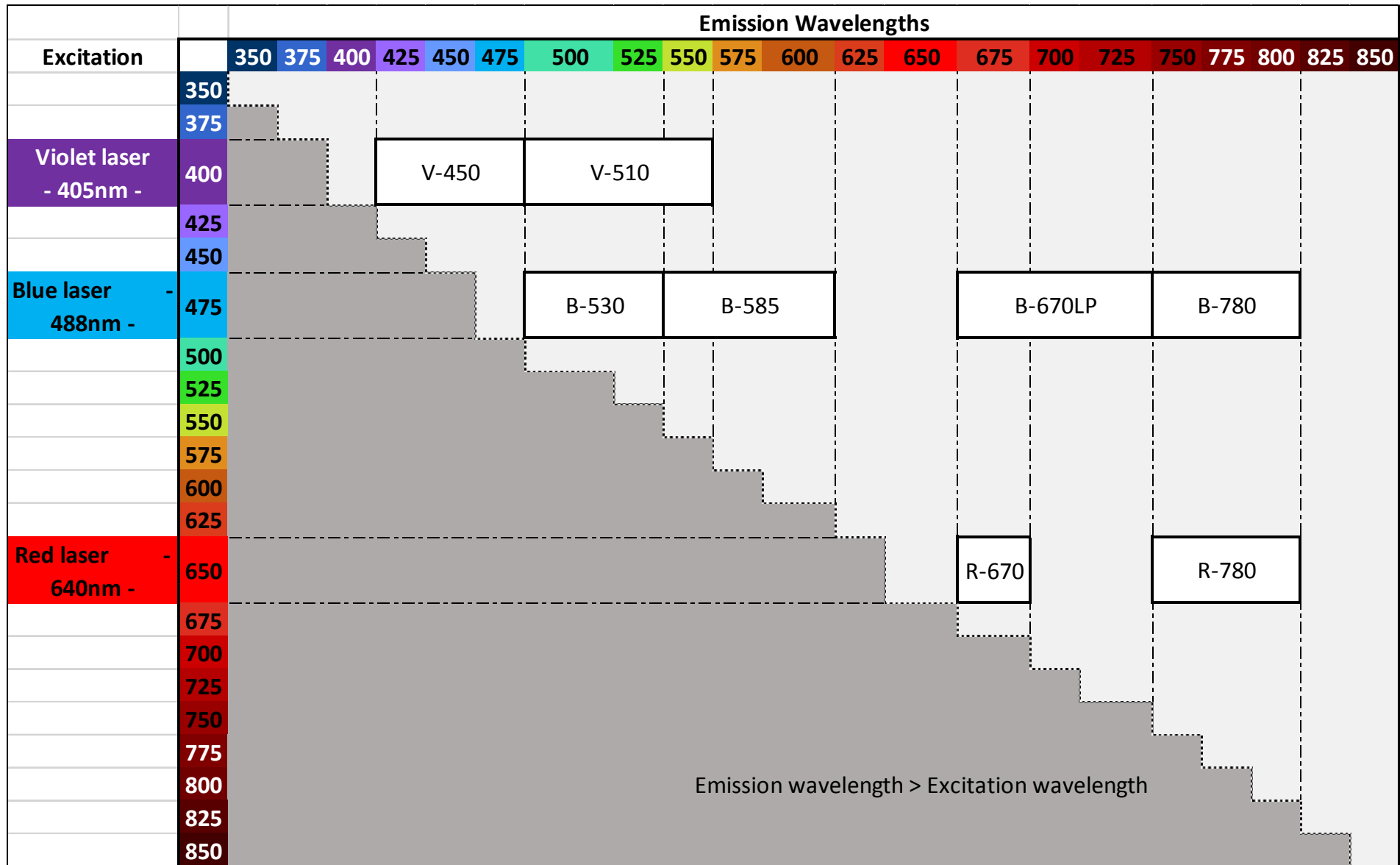
Greatest spectral spill-over & spread between horizontal & vertical (cross-laser) neighbouring detectors for a given wavelength
